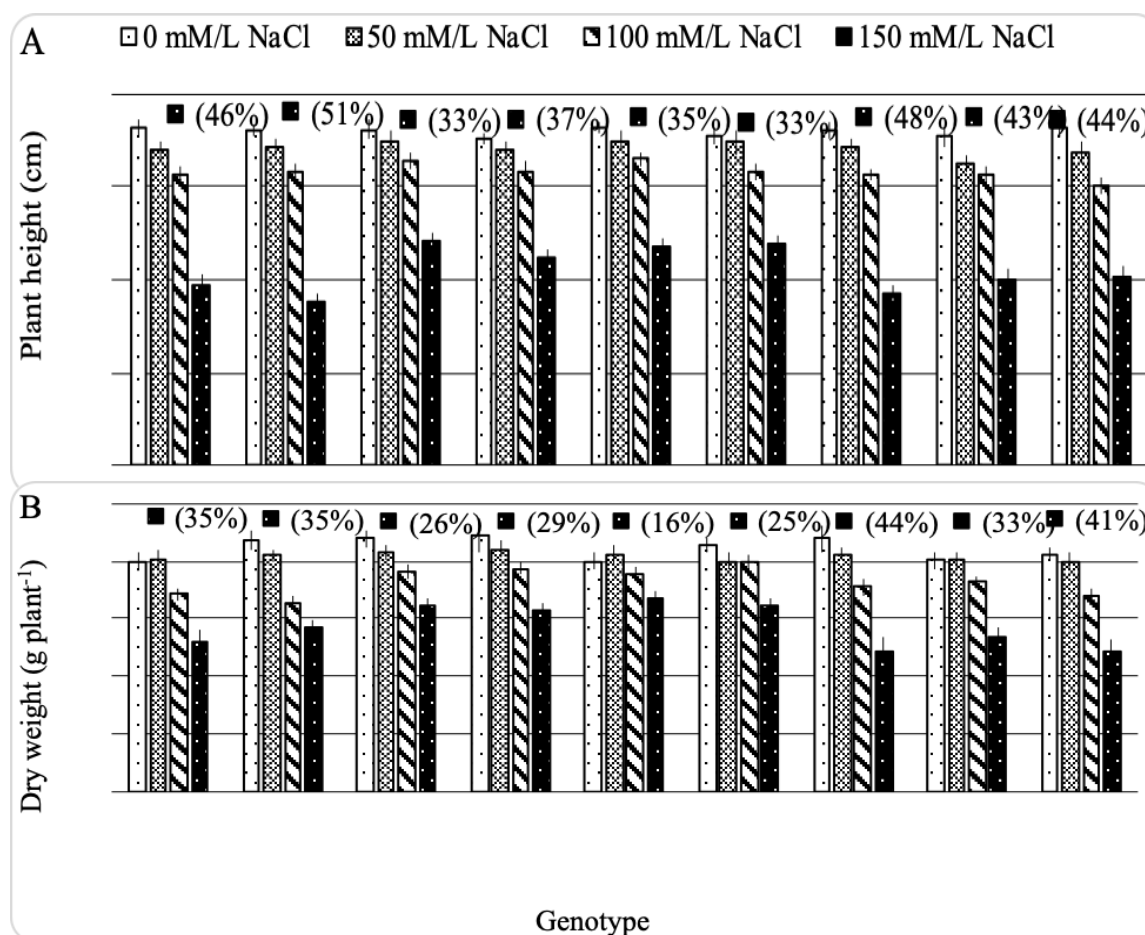
Figure 1: Effect of salinity on (A) plant height (cm) and (B) total dry weight (g plant -1 ) of 9 hard wheat genotypes. Values shown are mean ± SE. Values in parenthesis indicates the percent differences from 0mM NaCl to 150mM NaCl salinity treatment.
